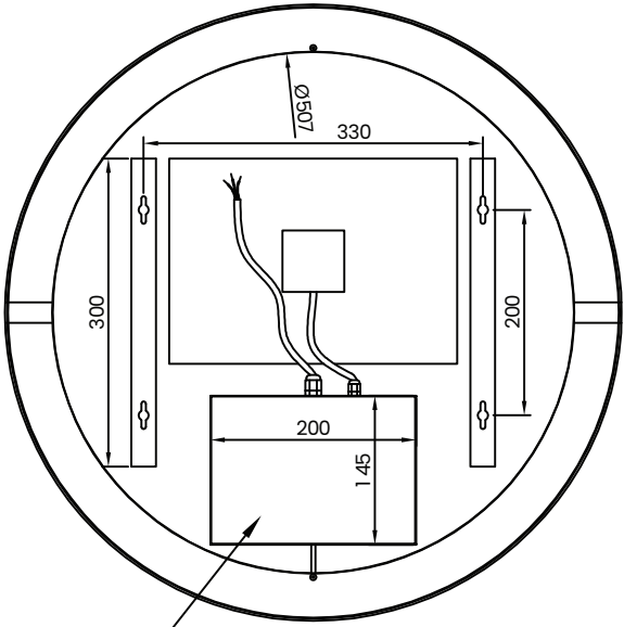
Electronic Box Back View
