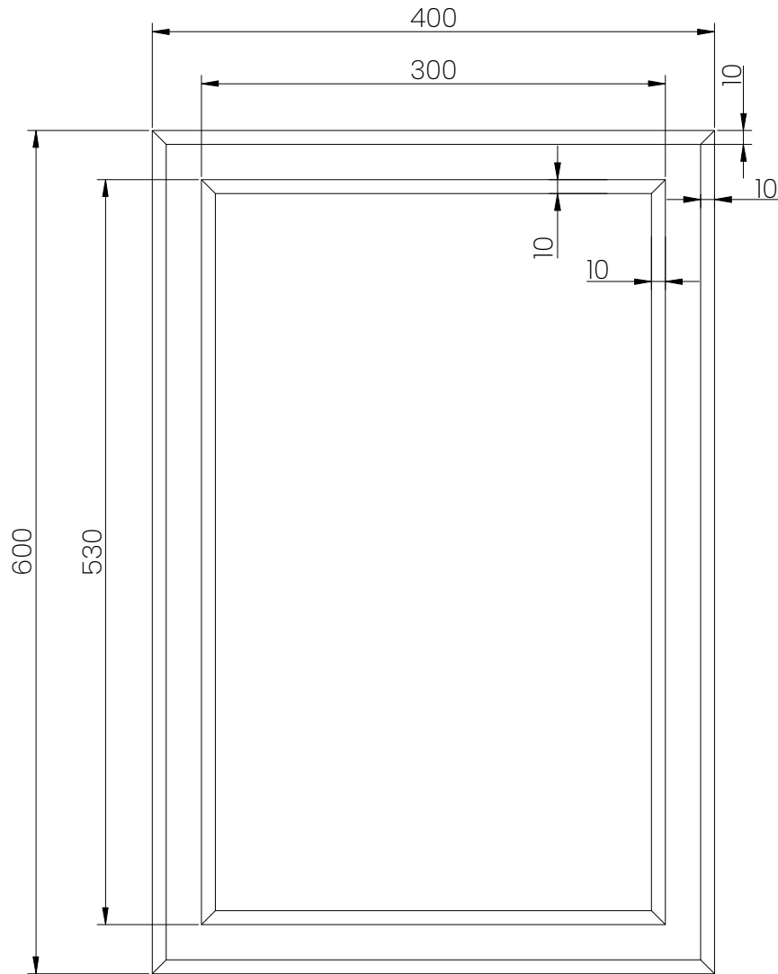
Front View
