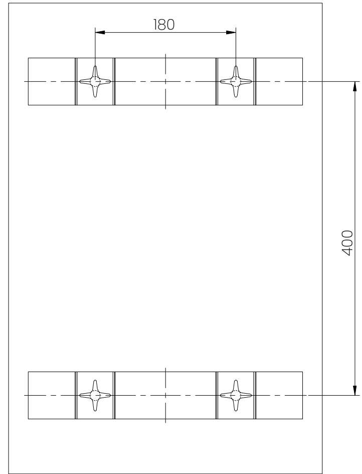
Back View
