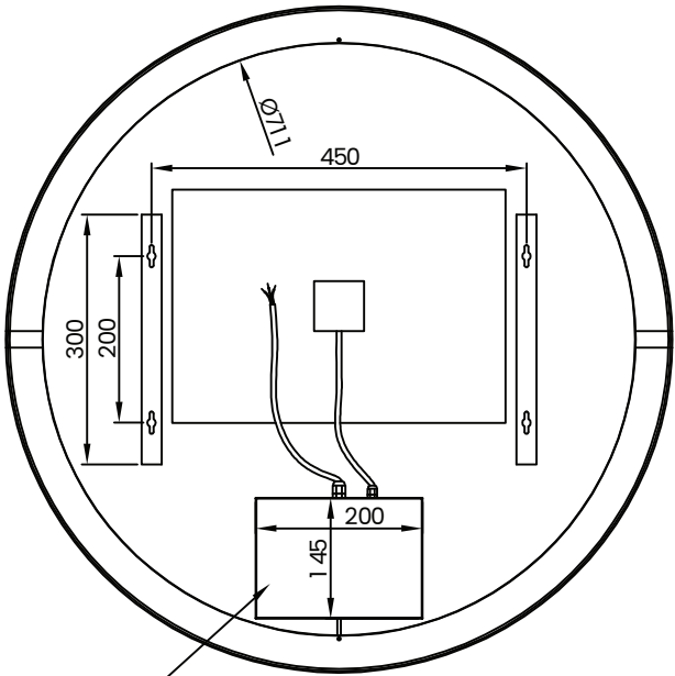
Electronic Box
