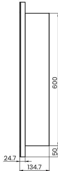
Right View
