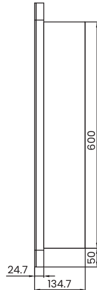
Right View
