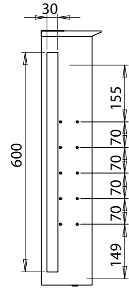
Left View
