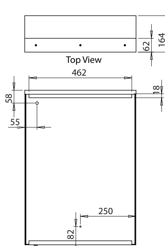
Bottom View
